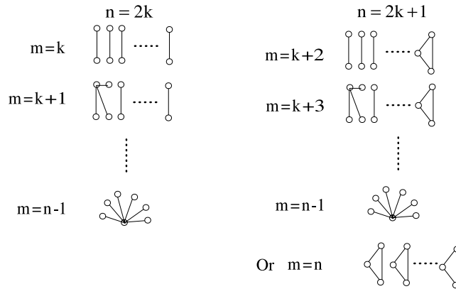
Fig. 1. Description of P_4 -saturated graphs.
