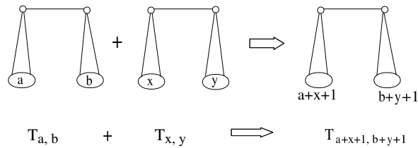
Fig. 3. The evolution of P_5 -saturated trees.
