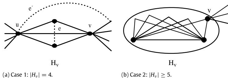
Fig. 4. The local structure of H_v .
