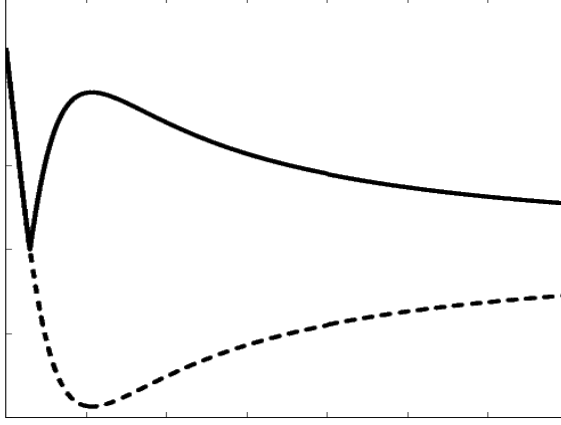
FIG. 4.1. \tilde{f} as a function of k .
