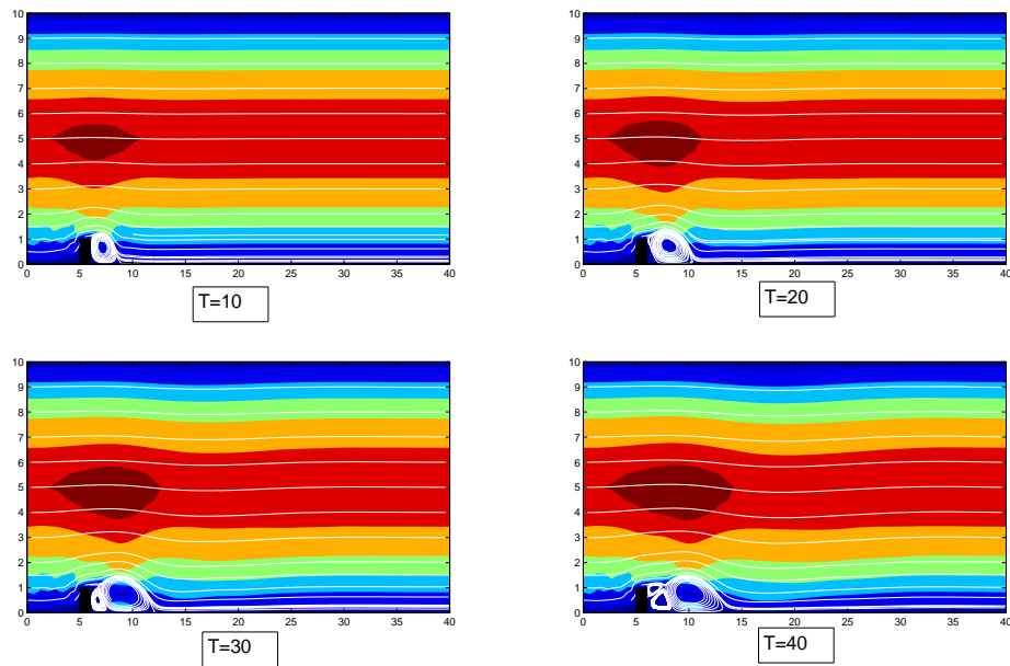
Figure 9: The above figure shows the velocity streamlines and speed contours for the coarse mesh solution of NS- \alpha with \alpha = 0.25 , \gamma = 1 and N = 1 . Shown is the solution at T=10, 20, 30 and 40 , which shows eddy formation and detachment, and a smooth resolved flow that matches the truth solution well.
