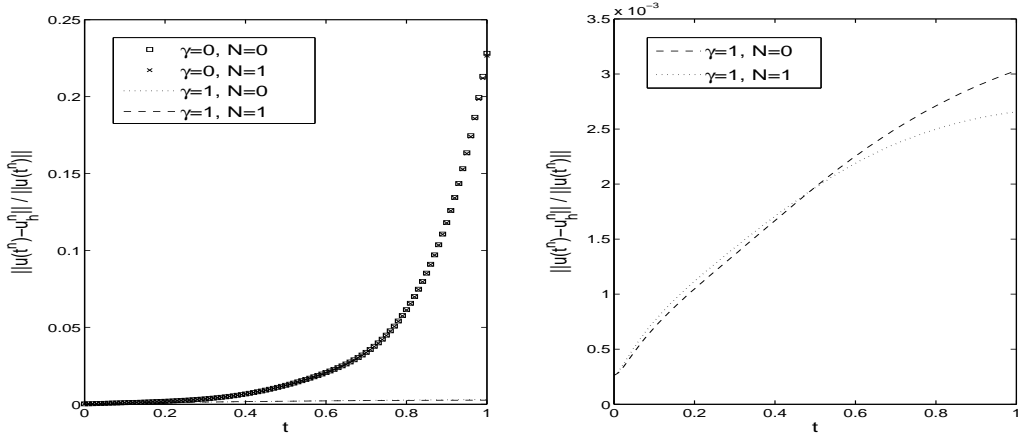
Figure 3: Relative L^2 error vs time in the numerical scheme for NS- \alpha studied herein, for the Eithier-Steinman problem with a = 1.25 , d = 1 , Re = 10,000 , \Delta t = 0.01 , with varying \gamma and N . The left plot shows the error from four schemes, but since the error when \gamma = 0 is so large, comparing the (\gamma = 1, N = 0) and (\gamma = 1, N = 1) schemes was impossible due to scaling. The plot on the right is thus the same plot, but without the error from the \gamma = 0 schemes.
