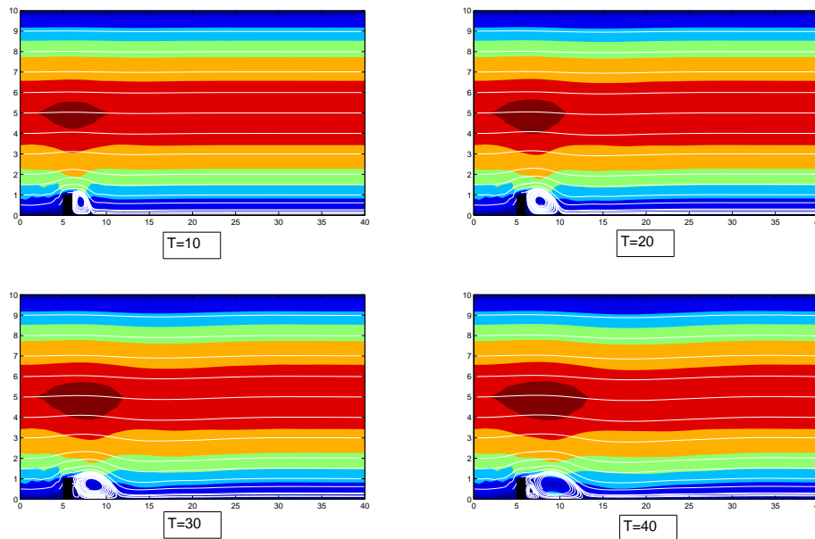
Figure 8: The above figure shows the velocity streamlines and speed contours for the coarse mesh solution of NS- \alpha with \alpha = 0.25 , \gamma = 1 and N = 0 . Shown is the solution at T=10, 20, 30 and 40 , which shows eddy formation and detachment, and a smooth resolved flow.
