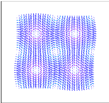
Figure 1: The velocity field and pressure contours of the Taylor-Green vortex decay problem at t = 0 .
