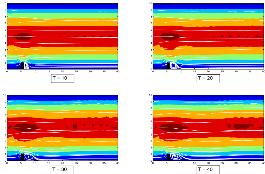
Figure 7: The above figure shows the velocity streamlines and speed contours for the coarse mesh solution of NS- \alpha with \alpha = 0.60 , \gamma = N = 0 . The extra regularization has damped much of the oscillations that destroyed the solution when \alpha = 0.25 (see Figure 6), but this amount of regularization prohibited eddy detachment.
