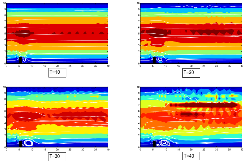
Figure 6: The above figure shows the velocity streamlines and speed contours for the coarse mesh solution of NS- \alpha with \alpha = 0.25 , \gamma = N = 0 . Shown is the solution at T=10, 20, 30 and 40 , which shows eddy formation and detachment, but reveals the flow is very under-resolved, as evidenced by the oscillations in the speed contours.
