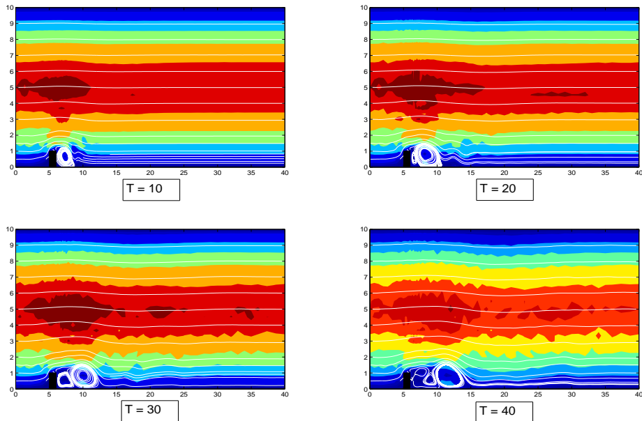
Figure 4: The above figure shows the velocity streamlines and speed contours for the coarse mesh solution of the NSE with the skew-symmetric form of the nonlinearity. Shown is the solution at T=10, 20, 30 and 40 , which is under-resolved, as evidenced by the oscillations in the speed contours.
