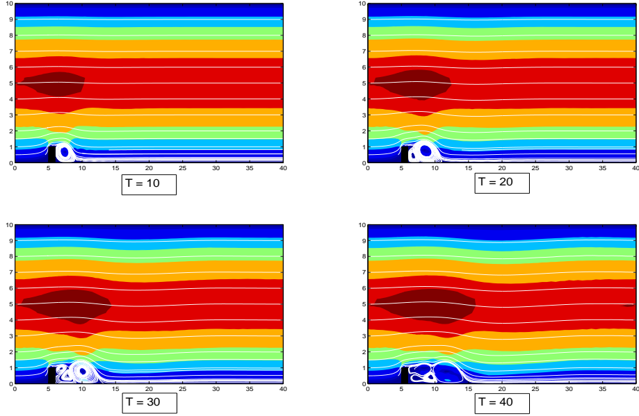
Figure 5: The above figure shows the velocity streamlines and speed contours for the NSE at T=10 , 20, 30 and 40 on the finer mesh. This is the “truth” solution for the test problem.
