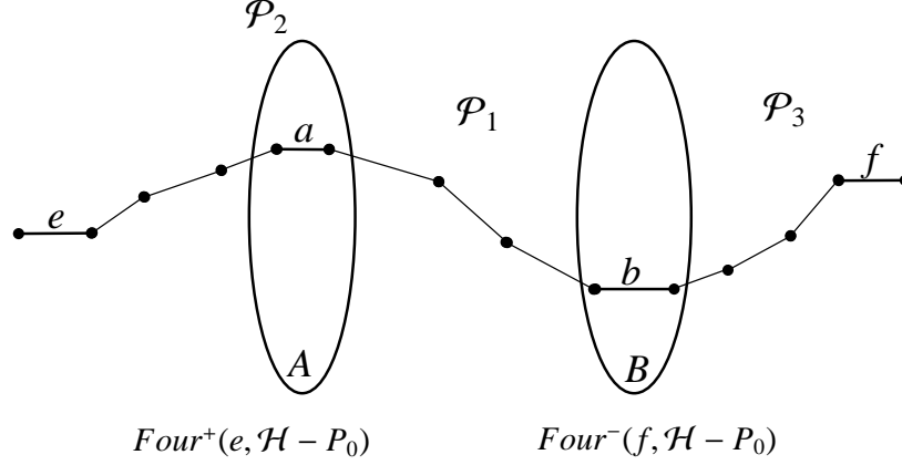
FIGURE 3. A hyperpath from e to f . (An illustration of the proof of Theorem 2.9)
