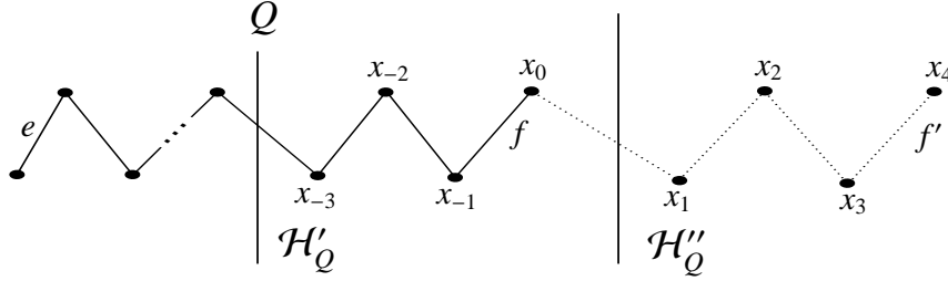
FIGURE 6. A hyperpath Q originating at e .
