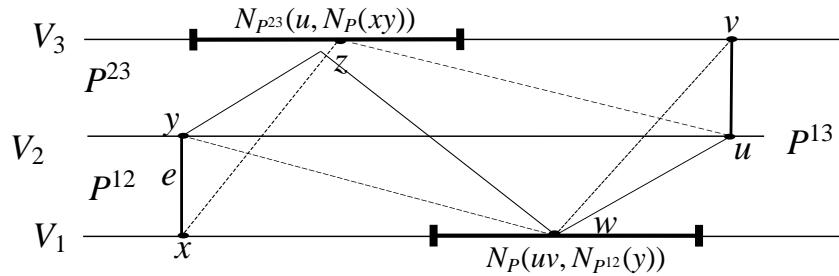
FIGURE 5. A hyperpath of length four originating at e = xy .
