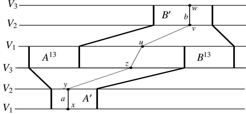
FIGURE 4. An illustration of the last case of the proof of Lemma 4.1.
