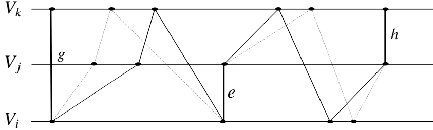
FIGURE 2. The fourth neighborhoods of e ( g \in Four^-(e, \mathcal{H}) , h \in Four^+(e, \mathcal{H}) ).
