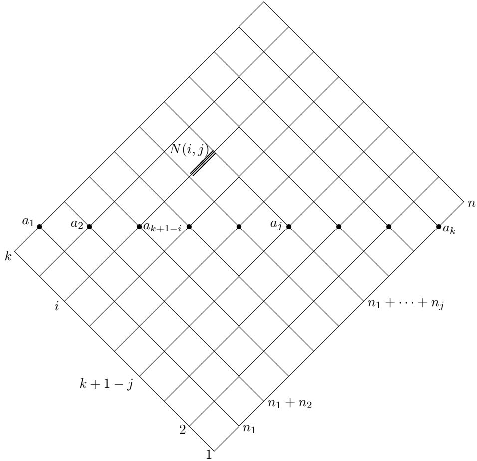
Figure 1: an interval N(i, j)
