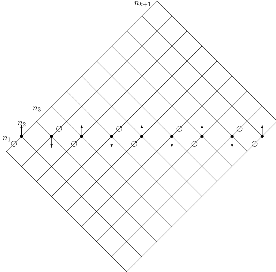
Figure 3: finding the capture vector of a_\uparrow
