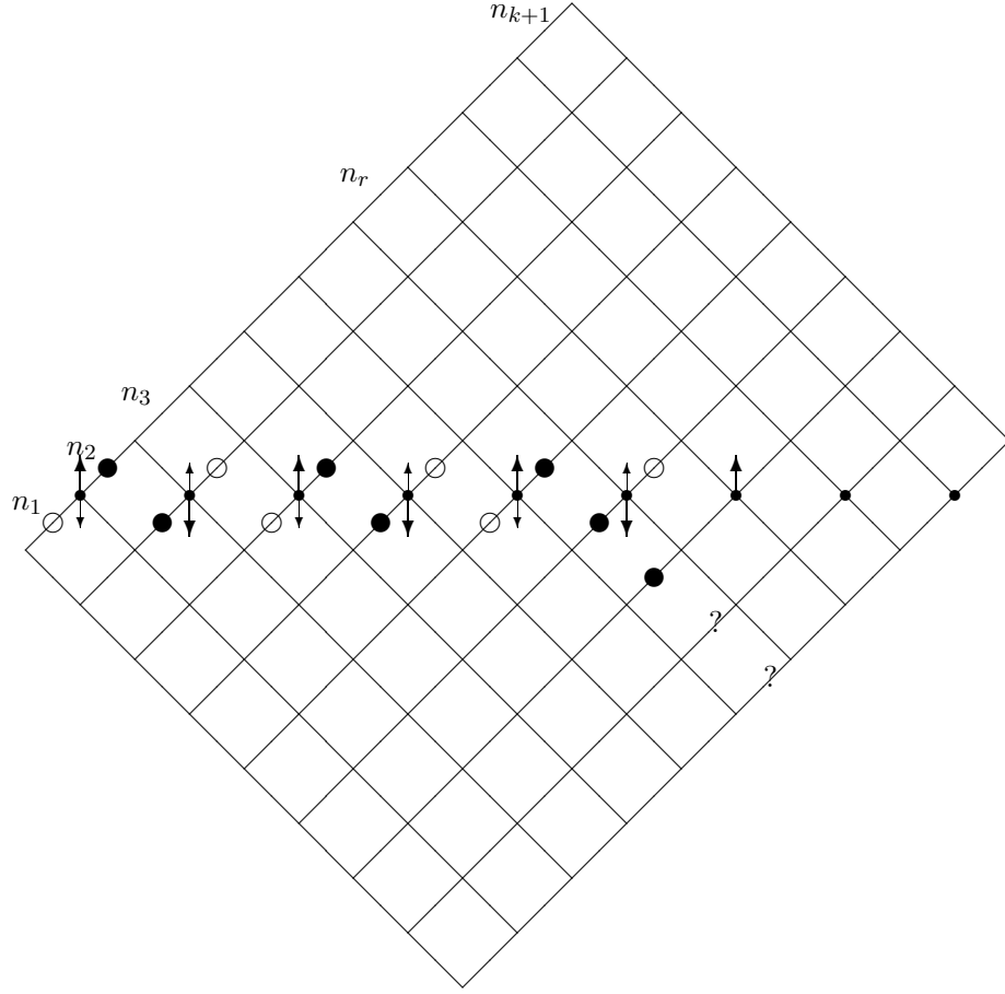
Figure 4: intervals lost and gained in switching from o to \hat{o}
